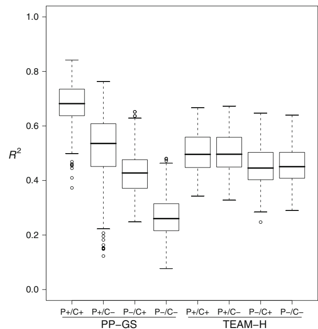
Fig. 1 Efficiency of prediction ( R^2 ) of grain yield for hybrids having no or one parental line evaluated in testcrosses. Prediction was based on estimates of general and specific combining ability (PP-GS) or combining abilities and AFLP marker data (TEAM-H). The underlying joint analyses of hybrids and parental lines were performed considering presence or absence of pedigree information (P+/P–) in combination with or without modeling the covariance between general combining ability and per se performance of parental lines (C+/C–). Each of the eight boxplot columns corresponds to a specific prediction scenario and comprises 300 R^2 values, which in cross-validation were obtained from observed and predicted performance of hybrids
