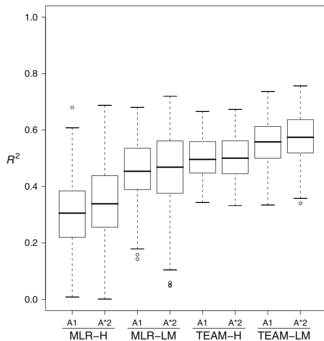
Fig. 2 Efficiency of prediction ( R^2 ) of grain yield for hybrids having no or one parental line evaluated in testcrosses. The marker-based prediction approaches (MLR-H, MLR-LM, TEAM-H, TEAM-LM) were applied to AFLP data pooling the two alternate classes of each heterozygous hybrid marker genotype (A1) and to imputed AFLP* data distinguishing the two alternate classes of each heterozygous hybrid marker genotype (A*2). Each of the eight boxplot columns corresponds to a specific prediction scenario and comprises 300 R^2 values, which in cross-validation were obtained from observed and predicted performance of hybrids
